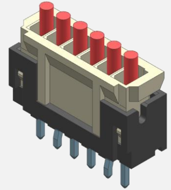
Mating View
